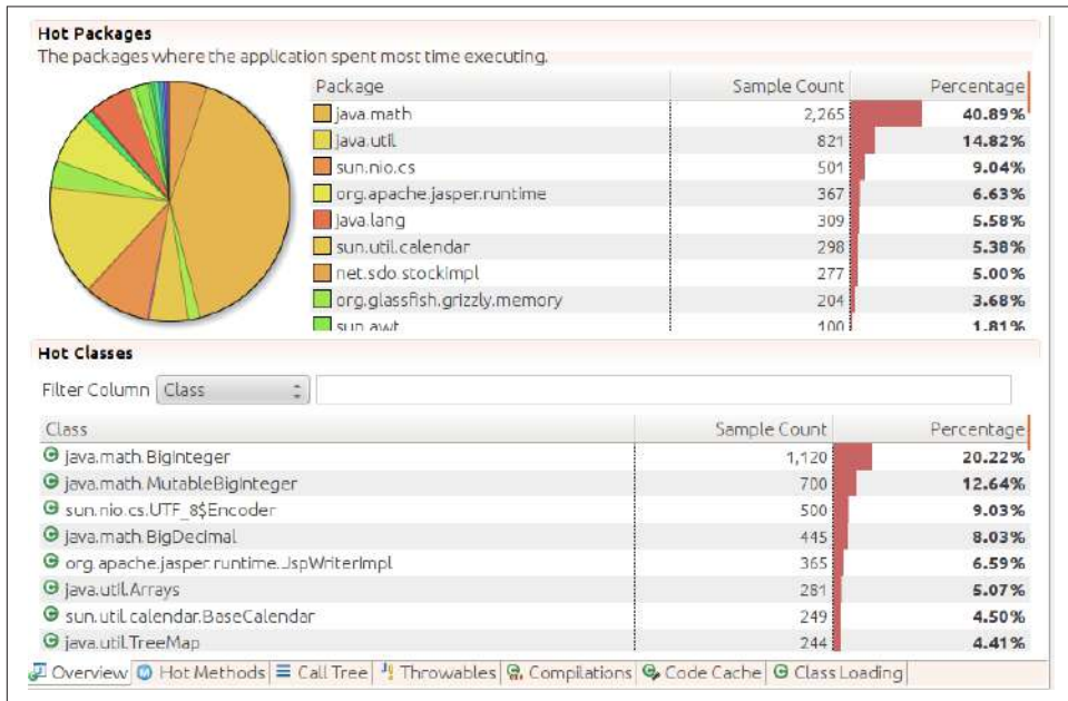
Figure 3-11. Java Flight Recorder Code panel
